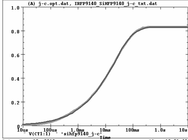
SiHFP9140 Tank j-c Temperature: 27.0
