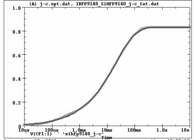
SiHFP9140 Filter j-c Temperature: 27.0
